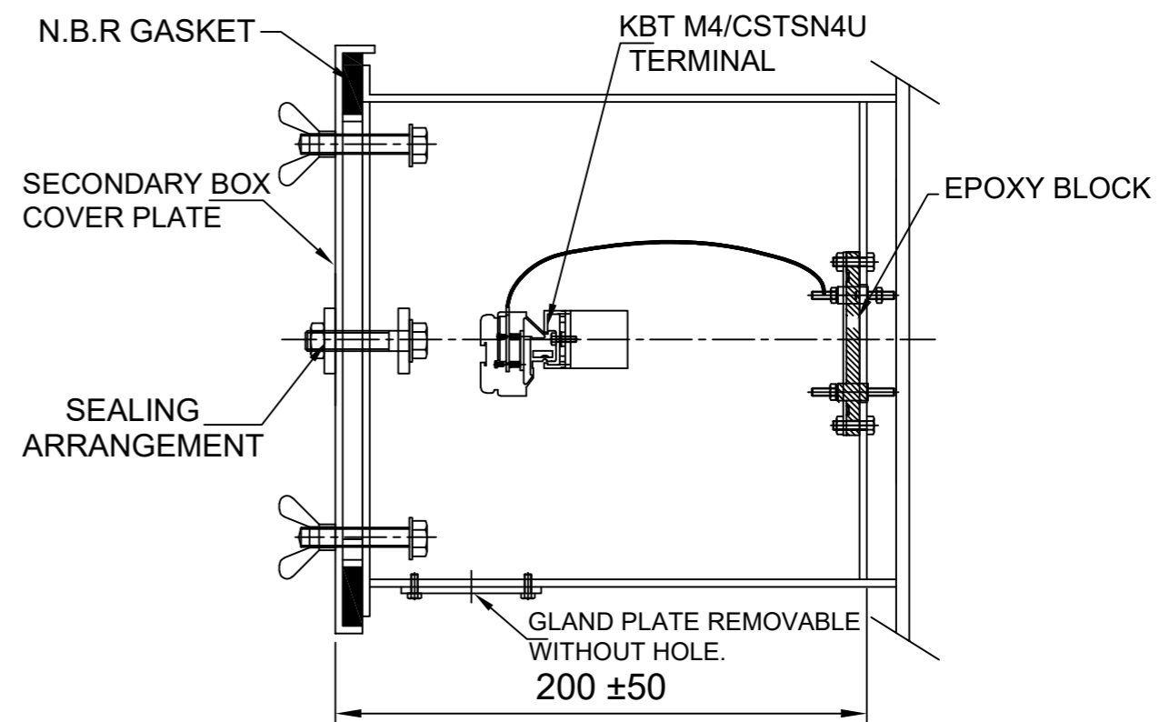
SIDE VIEW
