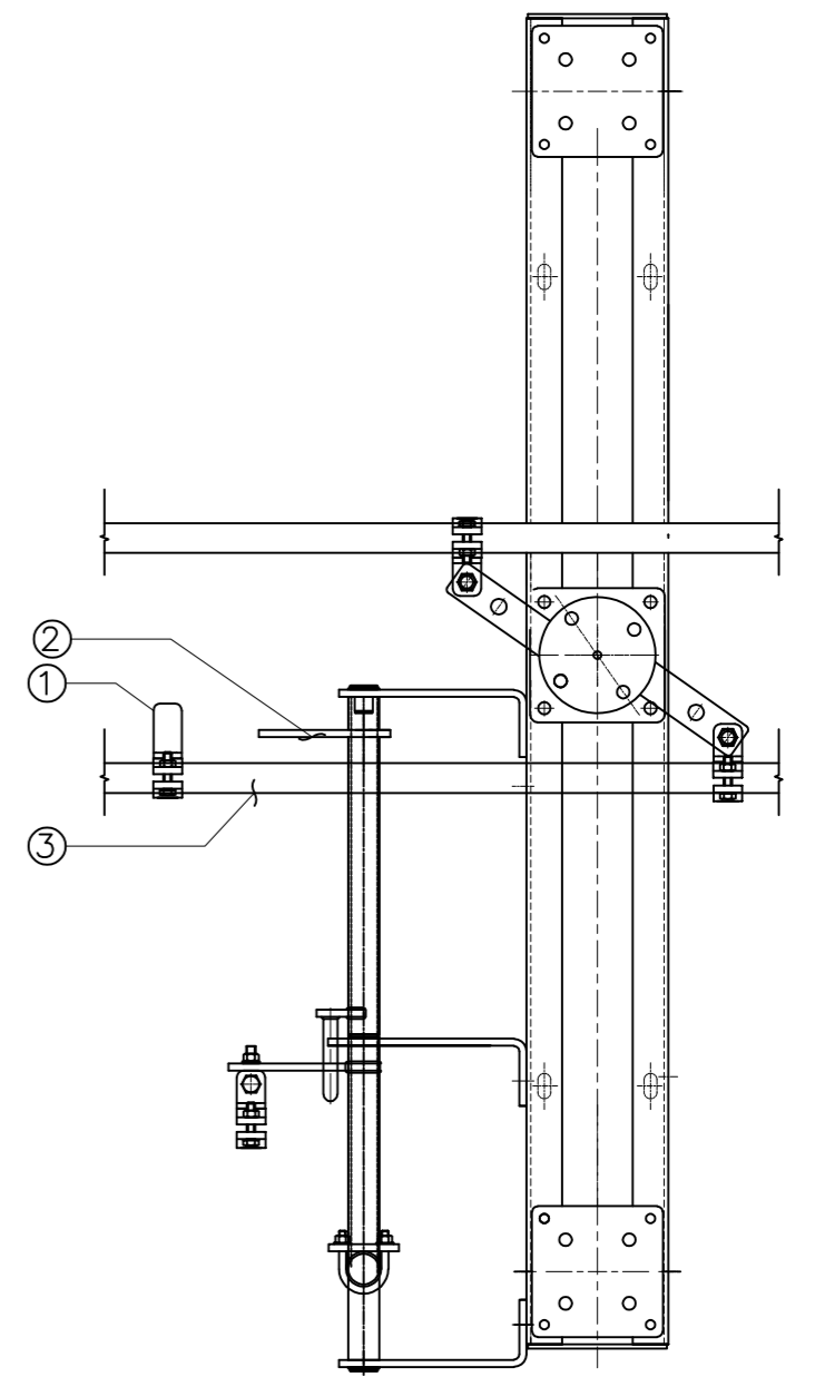
CASE- III ISOLATOR IN OPEN CONDITION & EARTH SWITCH IN CLOSED CONDITION
