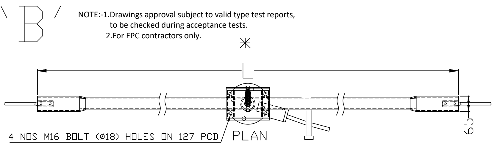
DETAILS OF FIXED CONTACT
