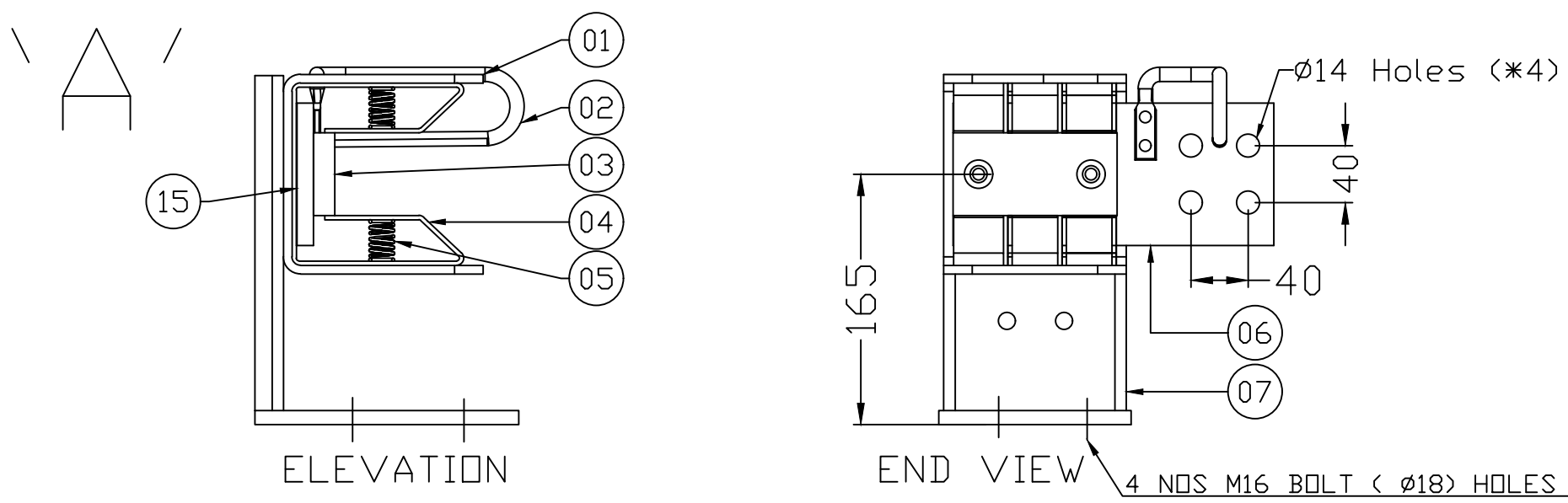
DETAILS OF FIXED CONTACT
