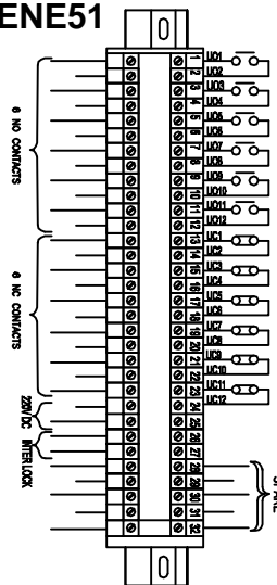
AUX. SWITCH CONTACT DETAILS FOR ISOLATOR (6 NO + 6 NC )
