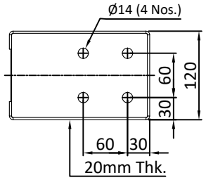
TERMINAL DETAIL
