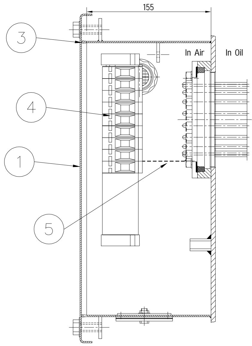
Section-AA
