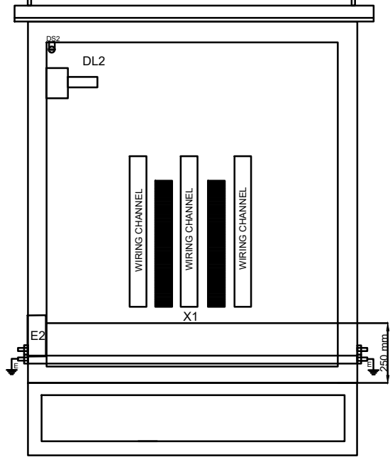
BACK VIEW ( DOOR OPEN ) ( TENTATIVE )
