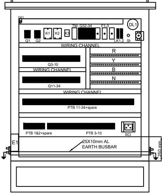
FRONT VIEW ( DOOR OPEN ) ( TENTATIVE )
