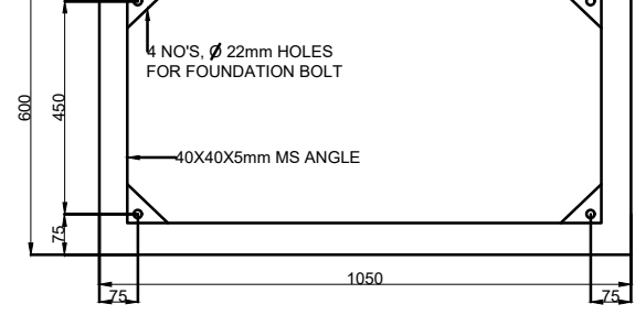
FOUNDATION PLAN
