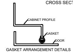
GASKET ARRANGEMENT DETAILS
