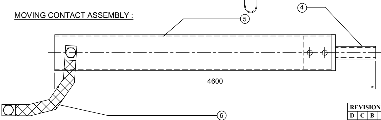
PLAN
