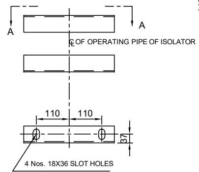
VIEW AT 'A - A'
