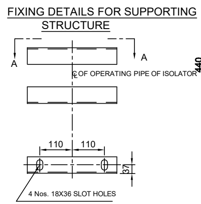
VIEW AT 'A - A'
