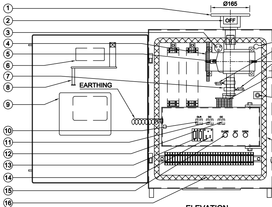
ELEVATION (DOOR IN OPEN CONDITION)
